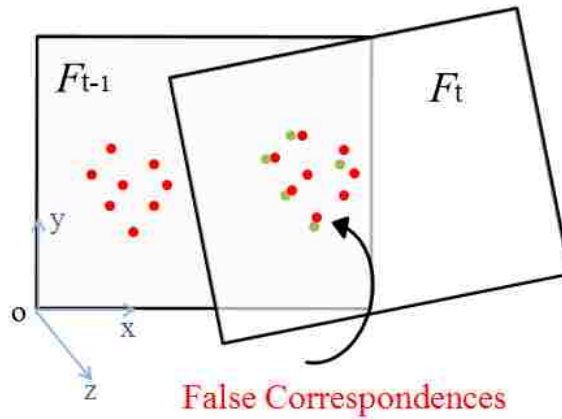
Figure 4.9: How ICP fails to align planar structures
