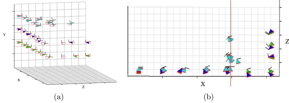
Figure 4.19: Camera pose estimation results: the ground truth is physically measured as the green cameras shows; the cyan cameras and blue cameras respectively indicate the results by [2] and our method.
